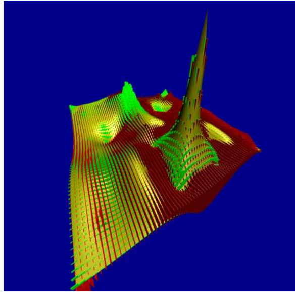
Figure 6: Cross-Hair glyphs
