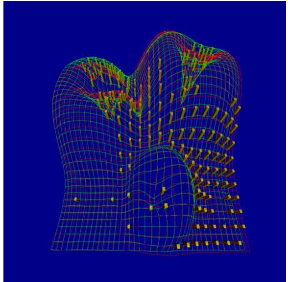
Figure 4: Displacement glyphs
