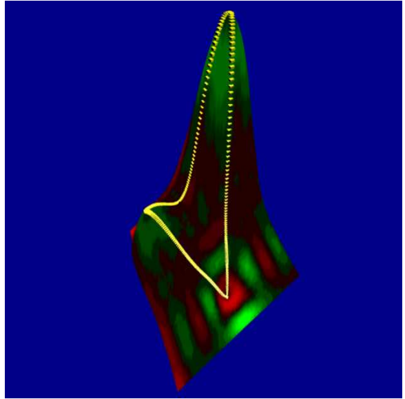
Figure 2: Swept probes
