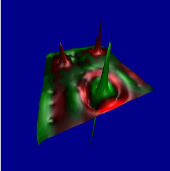
Figure 5: Pseudo-colored difference
