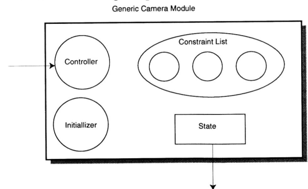
Figure 2: Generic camera module containing a controller, an initializer, a constraint list, and local state
