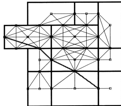
Figure 5: Room connectivity graph for the museum with a path found by A*
