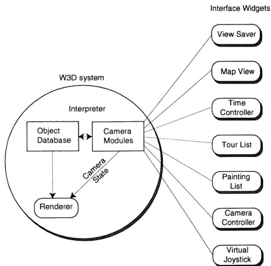
Figure 1: Overall Virtual Museum System
