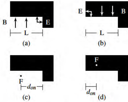
Figure 3: The properties of (a) entering and (b) exiting edge discontinuities: B - Discontinuity beginning. E - Discontinuity end. L - Discontinuity length. Arrow - Texel discontinuity ( d_c ). Black arrow - Entering discontinuity. White arrow - Exiting discontinuity. The relative position of the fragment F for entering (c) and exiting (d) edge discontinuities is defined by the parameter d_{on} , which is oriented towards the discontinuity end.
