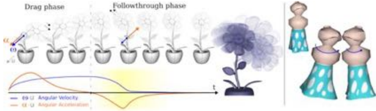
Figure 1: Real-time cartoon-like deformation computed automatically with Acceleration Skinning extending the range of deformation available from velocity only. Left: The joint use of angular velocity \omega and acceleration \alpha allows a smooth variation between an acceleration phase (where \omega and \alpha have the same orientation) associated with a drag effect, and a deceleration phase (where \omega and \alpha have opposite signs) associated with a “followthrough” transition. Right: A centrifugal effect coupled with a lift deformer creates the lift of the rotating skirt of this dancing toy character.
