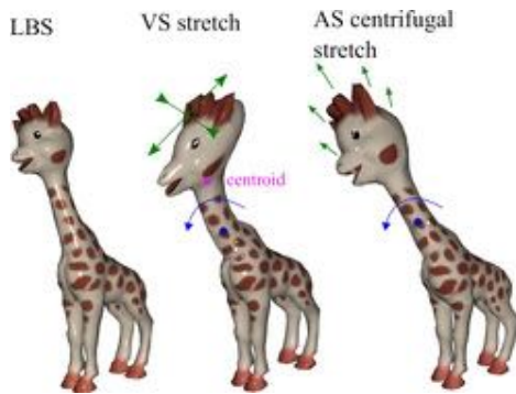
Figure 13: Comparison between VS stretch and AS centrifugal stretch deformer effects. Green arrows indicate the direction of stretch for rotation about the blue pivot. VS stretch also requires the notion of a centroid (pink) as well as a frame that depends on the bone orientation. Both capture distinct effects. VS stretch model cartoon squash and stretch to suggest the intensity of the speed of the motion. In contrast, AS centrifugal stretch models elongation, as if due to material yield by representing the centrifugal effect of bone rotation.
